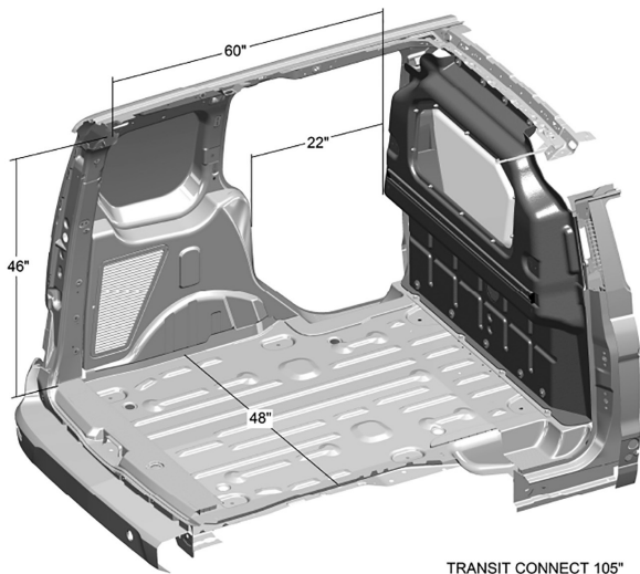
TRANSIT CONNECT 105"
